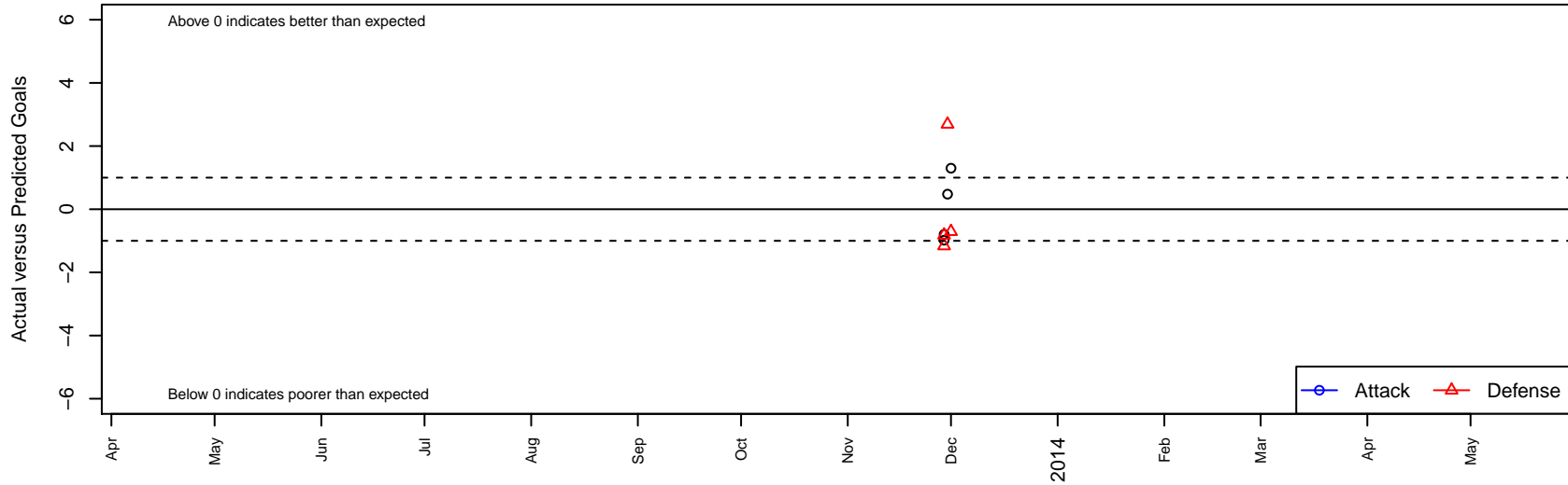
Downtown LVSC 03 Academy B02 Dots are actual minus expected GF (blue circles) and GA (red triangles). Blue line is smoothed change in attack strength. Red is smoothed change in defense strength.
